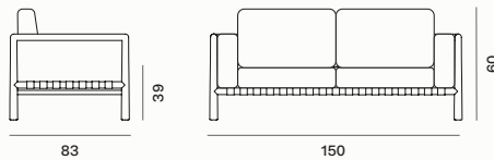
Sofa 2 seats / Divano 2 posti / Canapé 2 places
