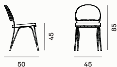
Chair / Sedia / Chaise ARISED
